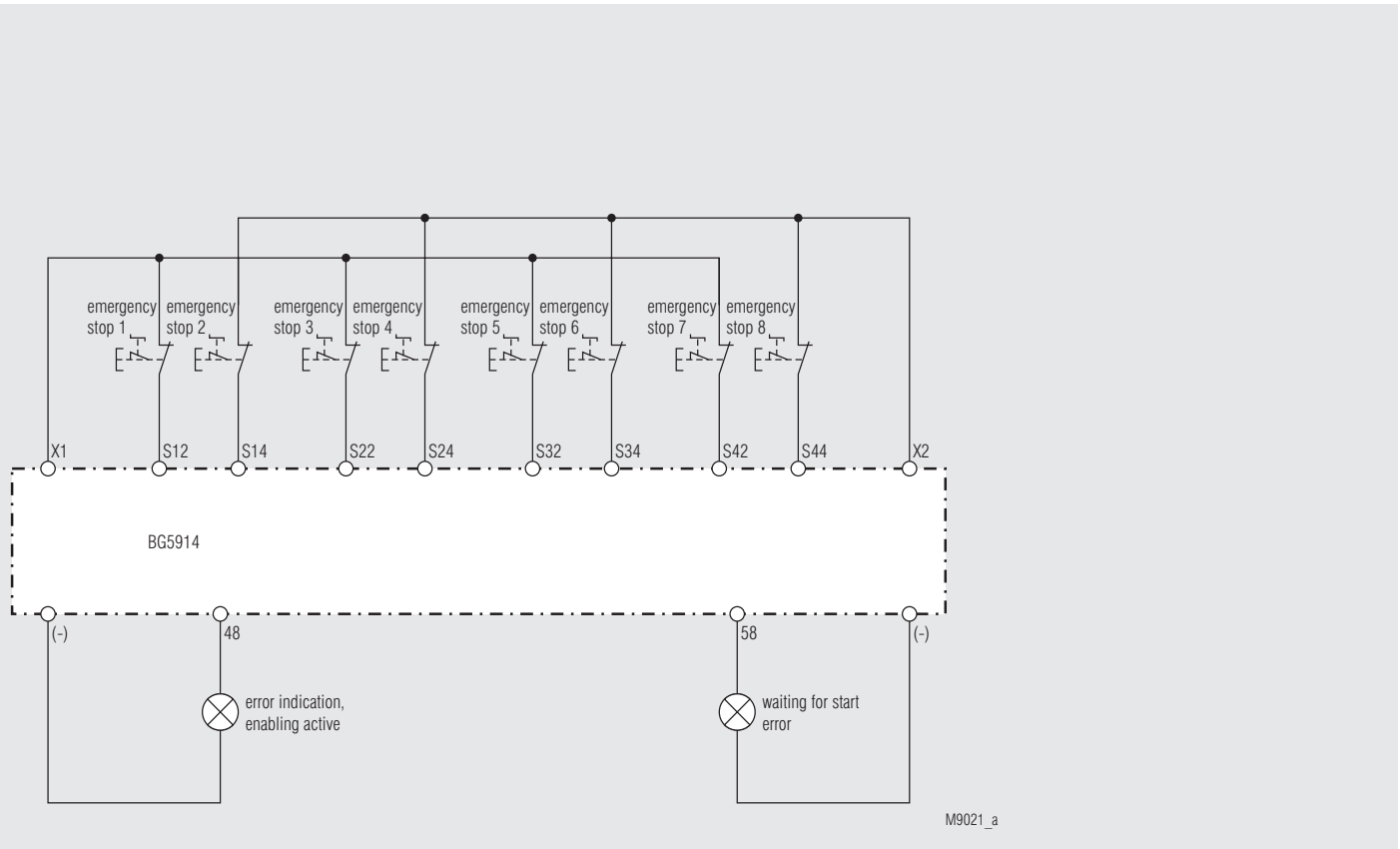
BG 5914, 8 Emergency stop, single-channel, voltage-free contacts; functions: 0 or 4
