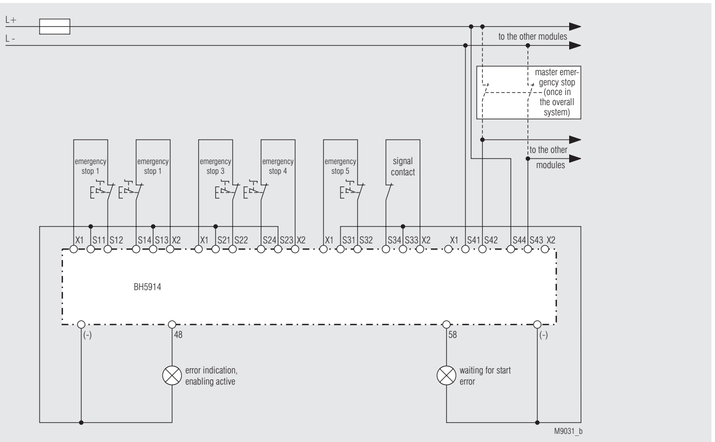
BH 5914, 5 Emergency stop single-channel + 1 Master Emergency stop 2-channel with short-circuit detection by means of wiring + 1 signal contact; functions 3 or 7
