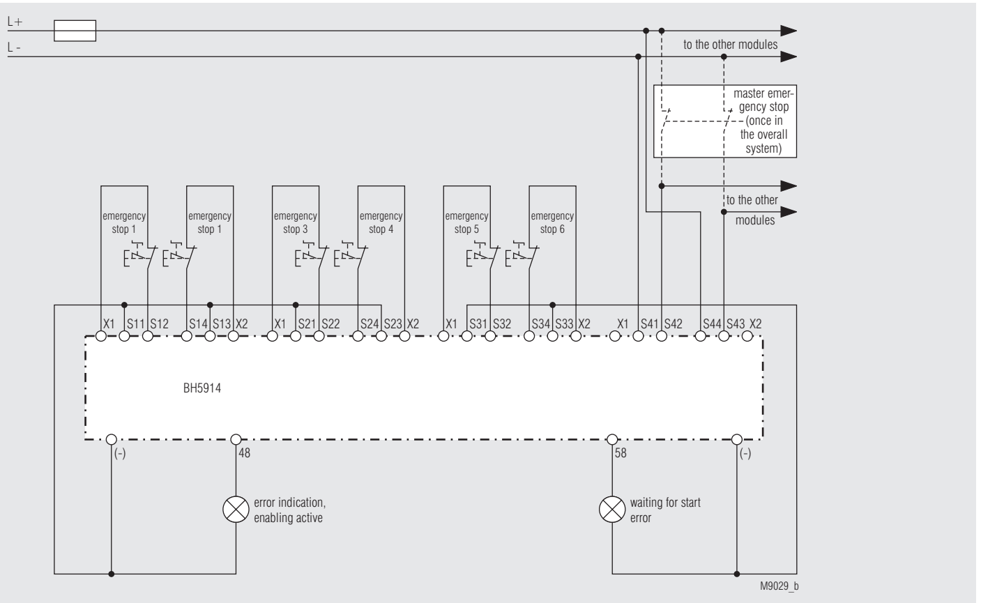
BH 5914, 6 Emergency stop single-channel + 1 Master Emergency stop 2-channel with short-circuit detection by means of wiring; functions: 2 or 6
